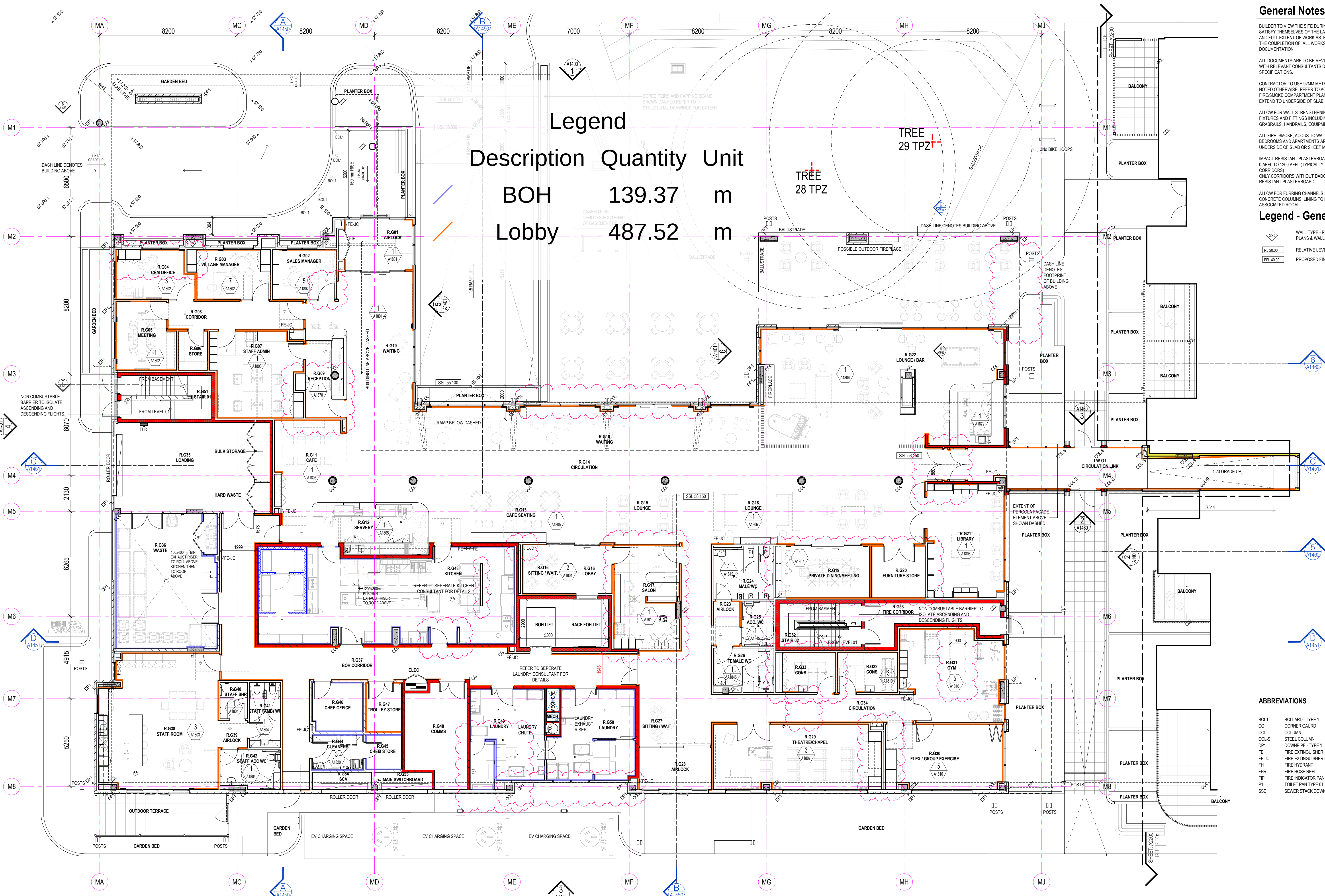
3 GROUND FLOOR PLAN - RACF Scale 1:100
